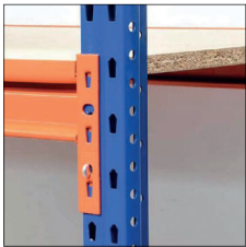
Slot in frames secured with locking pins
