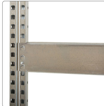
C70 Beams
