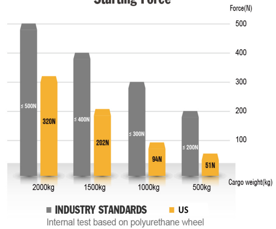
Starting Force
